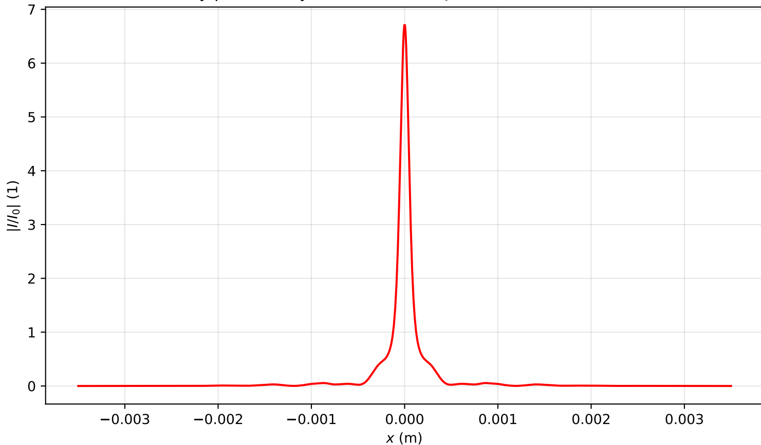
Intensity profile I(x, y = 0, z = 1.911)/I_0 , P_{in}=4.5P_{cr} , artificial time
